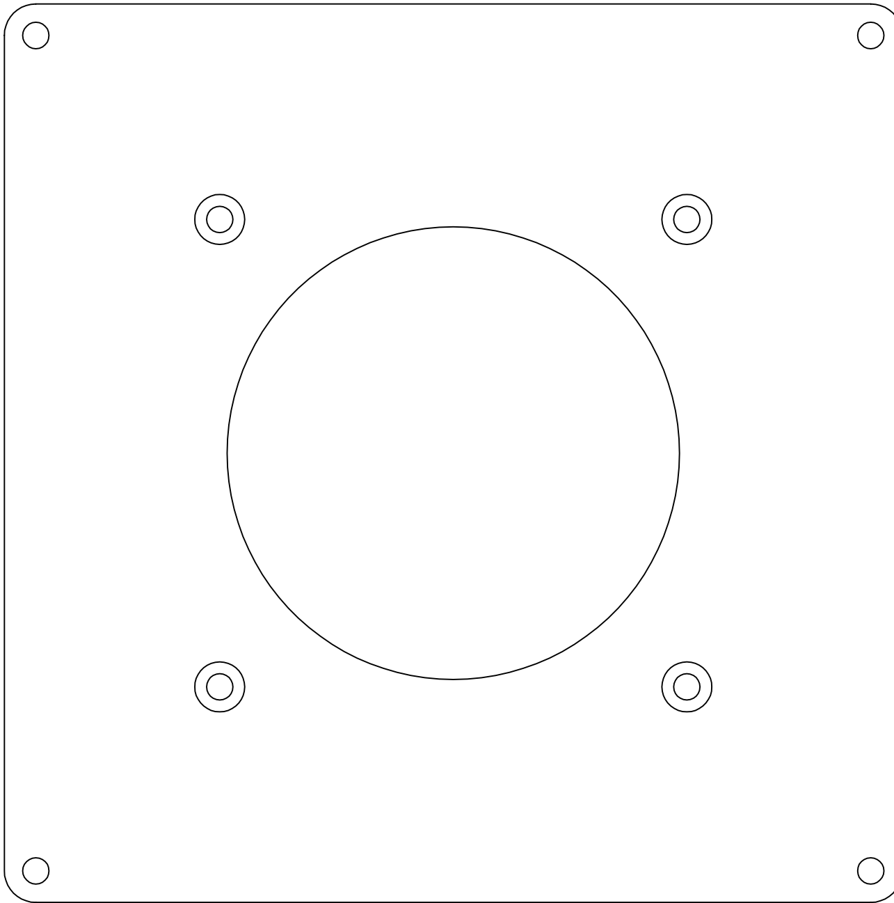
BSP-1L 170 x 170mm to suit 720 battery switches 1:1 when printed A4
