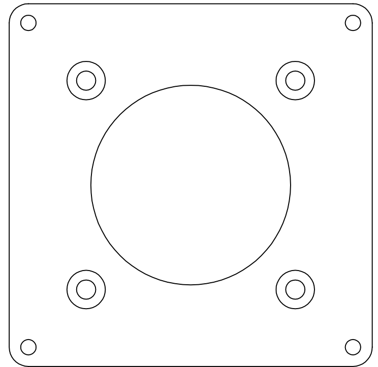
BSP-1 95 x 95mm to suit 701 battery switches 1:1 when printed A4
